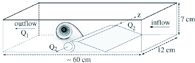
Fig. 1. Schematic of the experiment (from [2]). The vortex initiated by the step (5 mm high) is strained by the channel flow Q_1 and intensified and stretched by the axial suction Q_2 . The values Q_1 = 12.5 L/min and Q_2 = 7.5 L/min (i.e. the total flow rate through the channel = Q_1 + 2Q_2 .) were chosen to produce an intense quasi-periodically bursting vortex
