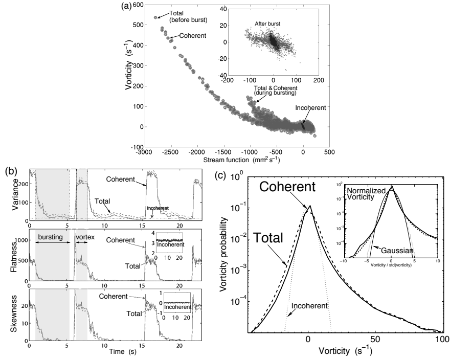
Fig. 3. (a) Scatter plot of the stream function versus vorticity showing the coherence of the vorticity field. The total and coherent are nearly indistinguishable while the incoherent remains localized at the origin. The inset shows the fields after the burst. (b) Time evolution of the moments of the vorticity field. Plotted are the variance (top), flatness (middle) and skewness (bottom) of the total (dashed line), coherent (solid), and incoherent (dotted) fields during 24 seconds, capturing three bursting events. (c) Probability distribution functions of the vorticity of the fields during the bursting. The inset shows the fields renormalized by their standard deviation
