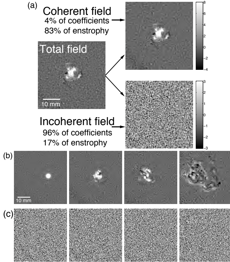
Fig. 2. (a) A split of the measured vorticity field into coherent and incoherent fields at the beginning of a burst. Each field snapshot has been renormalized by its standard deviation. (b) Time evolution of the coherent field and (c) incoherent field. Time proceeds from left to right in intervals of 0.33 seconds while the bursting vortex travels from right to left in the snapshots. The colormaps used for the coherent and incoherent fields are the same as in (a)
