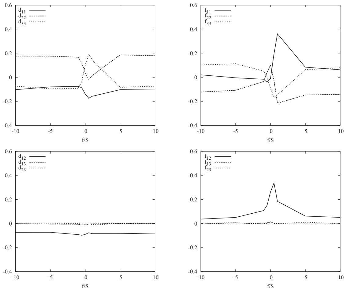
FIG. 7. Dependence of the diagonal components (top row) and off-diagonal components (bottom row) of the structure dimensionality anisotropy tensor d_{ij} (left column) and the circularity anisotropy tensor f_{ij} (right column) on the rotation ratio f/S at nondimensional time St=5 .
